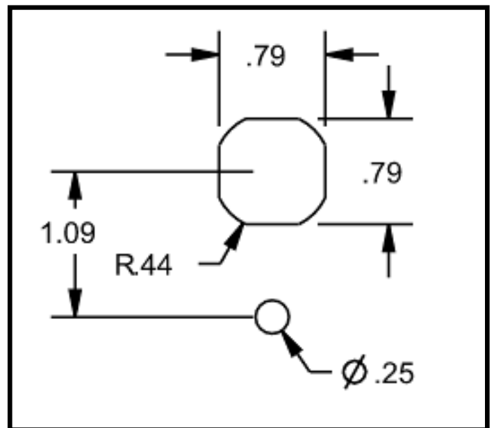
CUTOUT DETAIL
