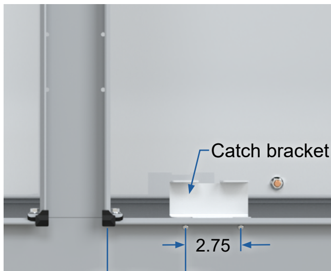
Latch bracket mounting hole location (typ. top and bottom flange)
