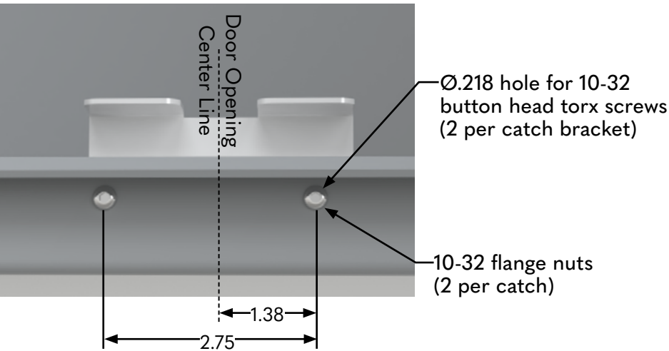
Section Y-Y
