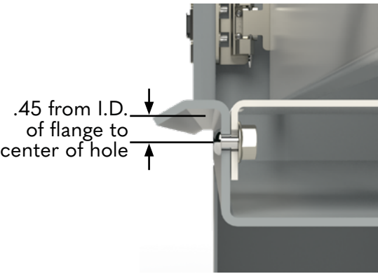
Section T-T
