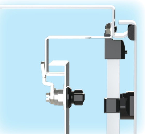
Section Z-Z
