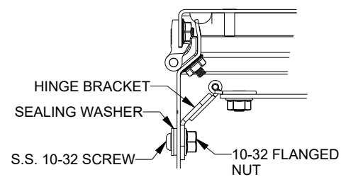
HINGE SIDE INSTALLATION DETAIL TYPICAL FOR ALL ENCLOSURES DO NOT SCALE
