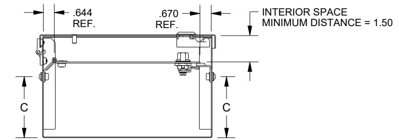
SECTION Z-Z
