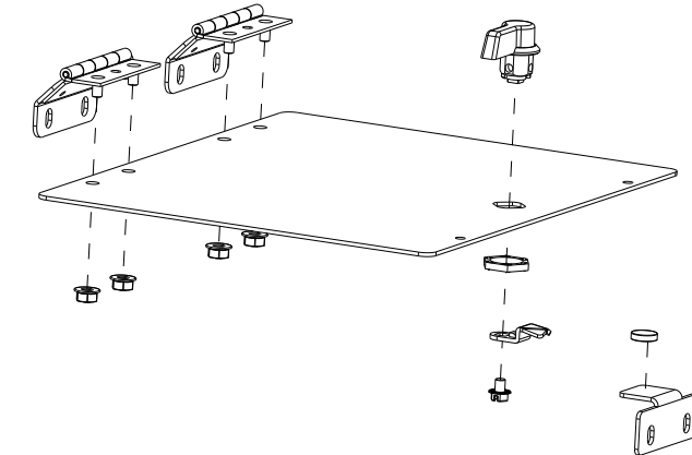
DEAD FRONT EXPLODED VIEW
