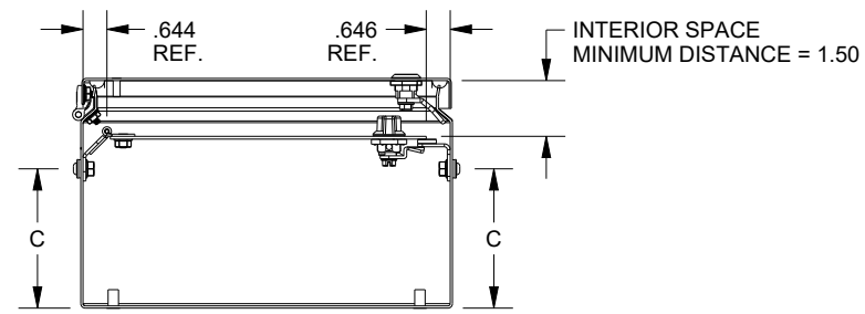
SECTION X-X
