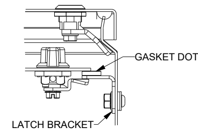
LATCH SIDE INSTALLATION DETAIL TYPICAL FOR ALL ENCLOSURES DO NOT SCALE
