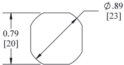
WING KNOB QT CUTOUT DETAIL
