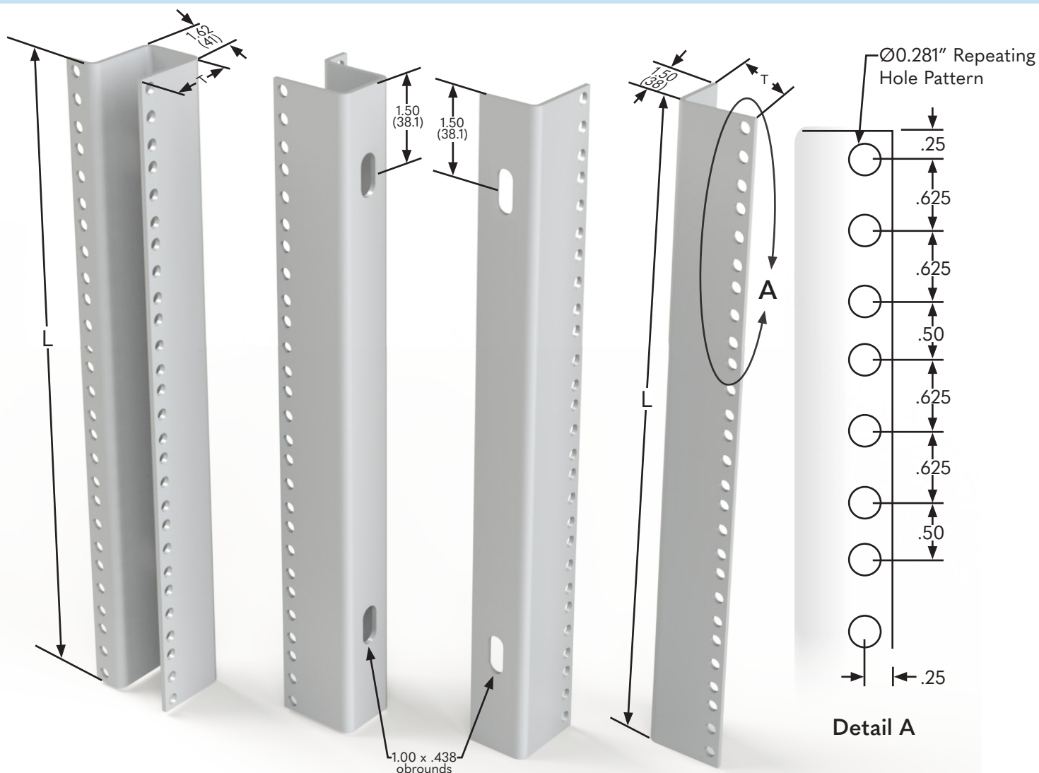
Rack Mounting Angle (Type RA)
