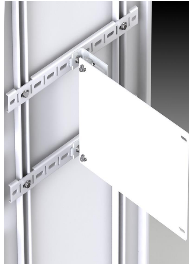
ASSEMBLED VIEW
