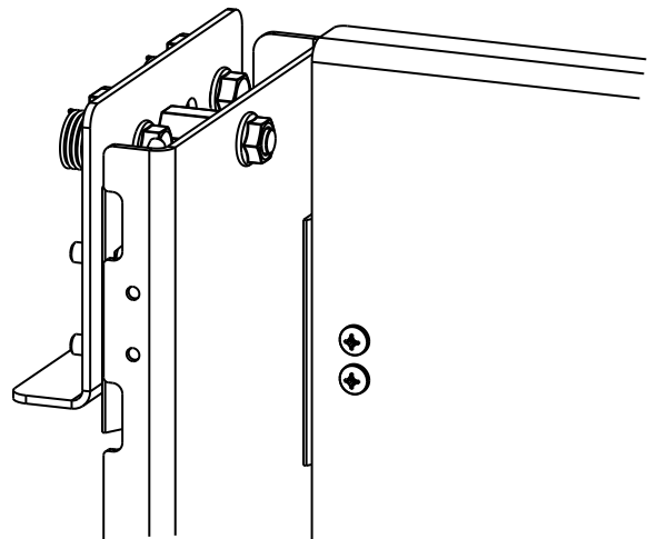
MOUNTING BRACKET & HINGE BRACKET FRONT ISOMETRIC NON-EXPLODED VIEW
