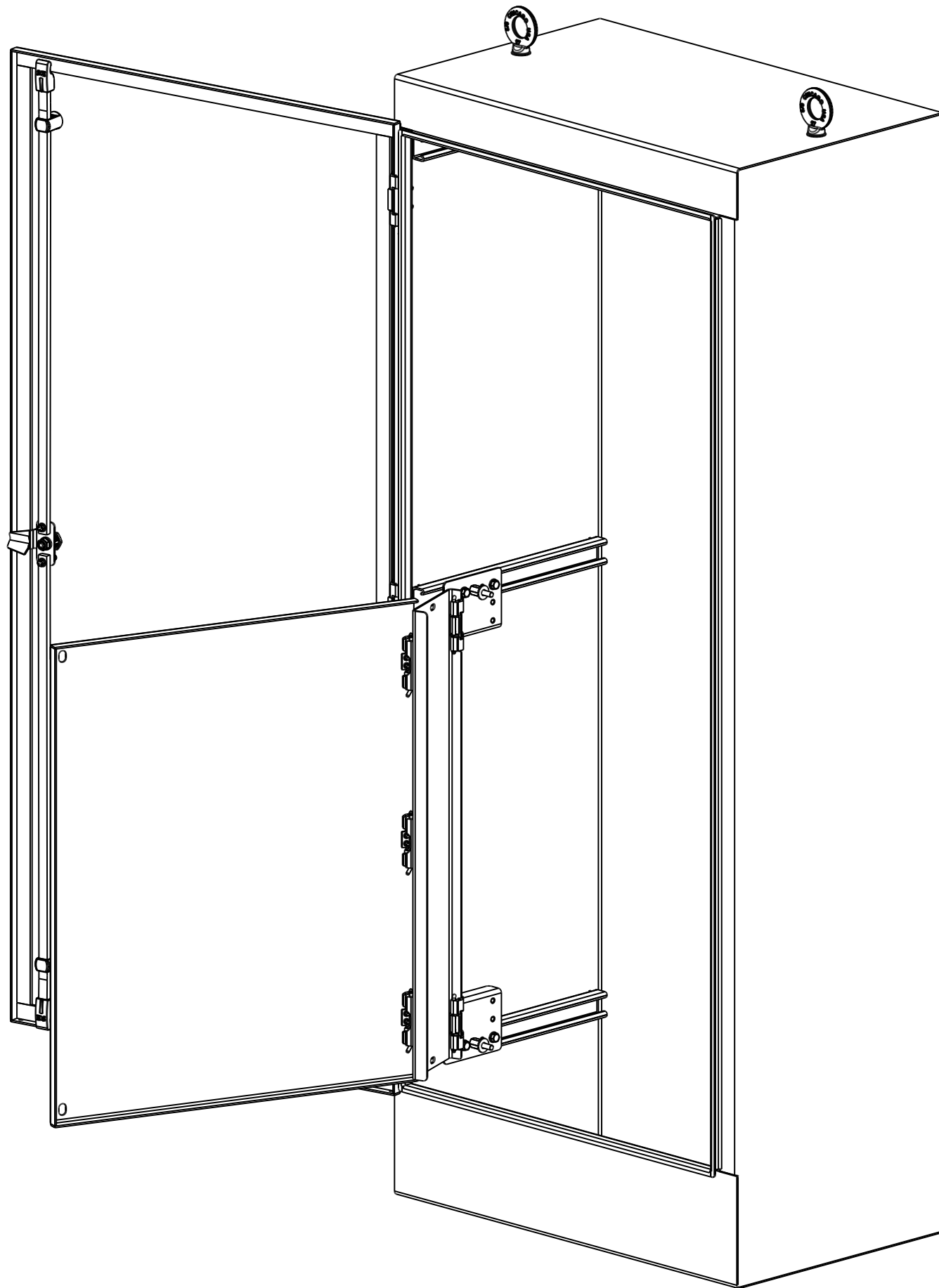
FRONT ISOMETRIC VIEW FOR REFERENCE SHOWING HALF SWING-OUT PANEL INSTALLED
