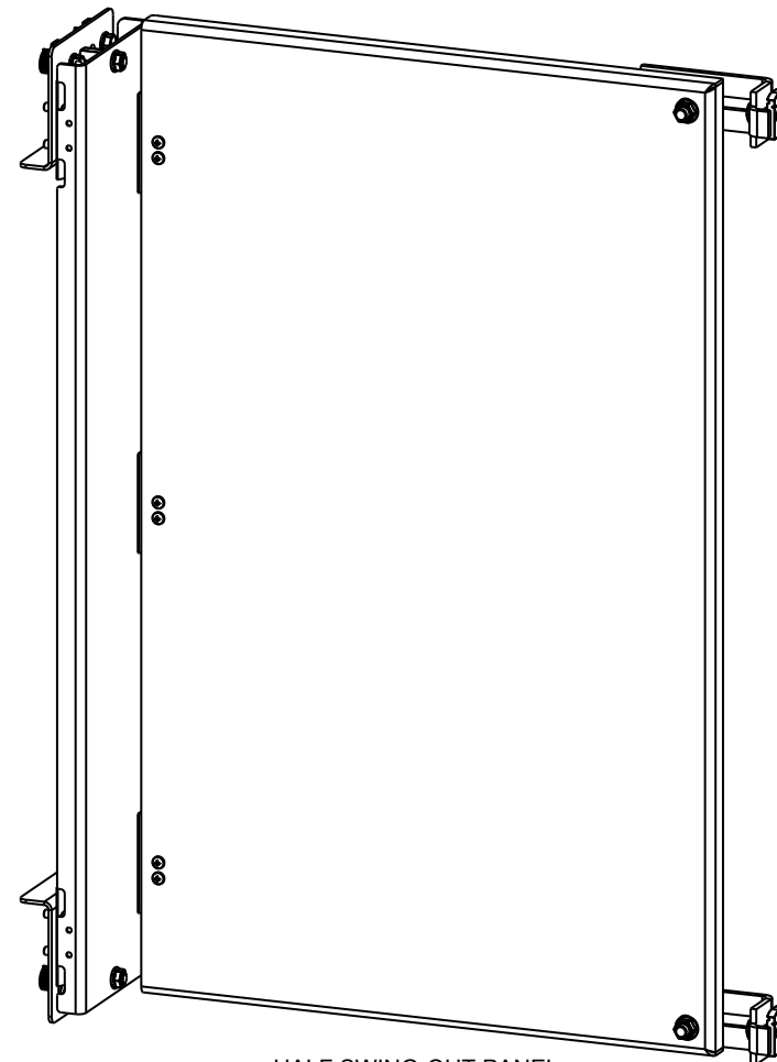
HALF SWING-OUT PANEL FRONT ISOMETRIC VIEW
