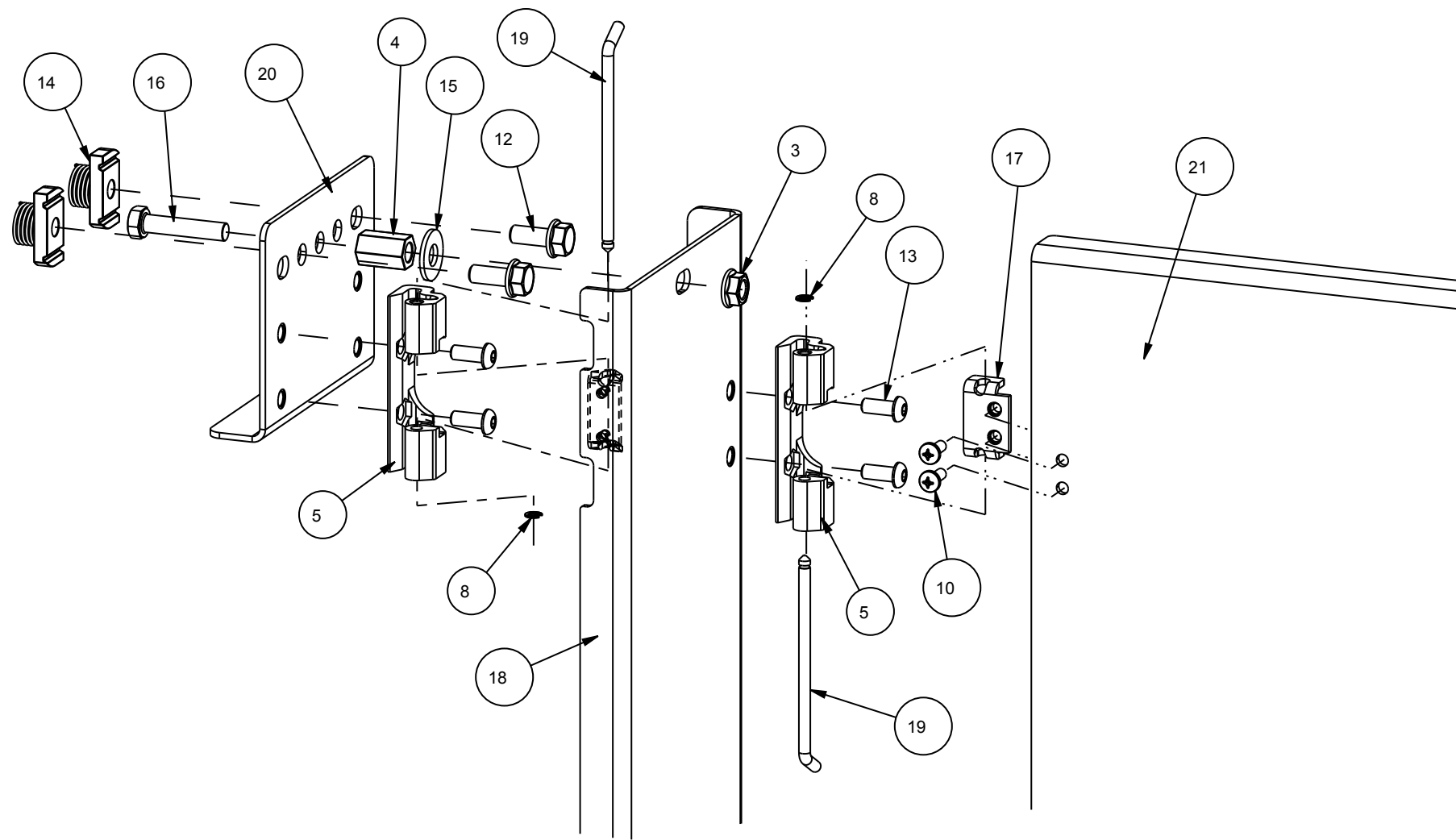
MOUNTING BRACKET & HINGE BRACKET FRONT ISOMETRIC EXPLODED VIEW
