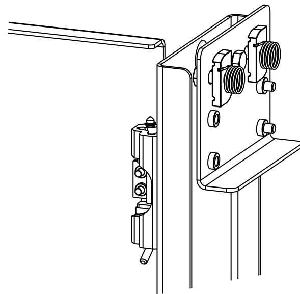
MOUNTING BRACKET & HINGE BRACKET REAR ISOMETRIC NON-EXPLODED VIEW
