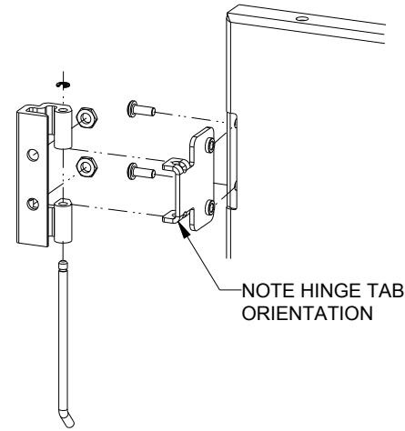
EXPLODED HINGE DETAIL
