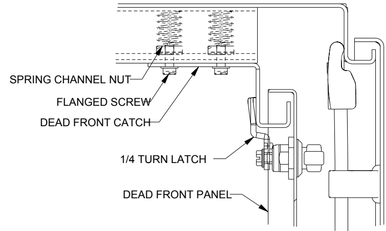
INTERIOR RIGHT SIDE SECTION VIEW
