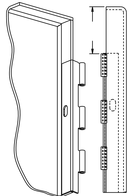
Bent Continuous Hinge (1st Knuckle on Door)
