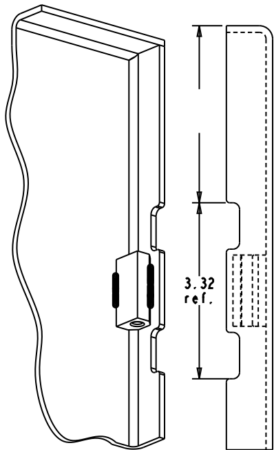
Large Concealed Hinge on 11ga. or 12ga. Door
