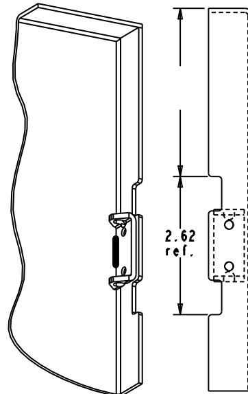
Small Concealed Hinge on 14ga. or 12ga. Door
