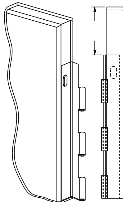
Bent Continuous Hinge (2nd Knuckle on Door)
