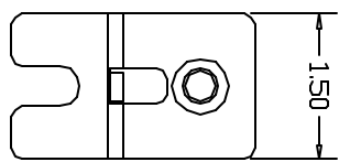
BOLT ON MOUNTING EAR (BOTTOM)
