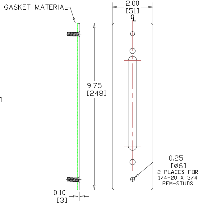
ADAPTER PLATE
