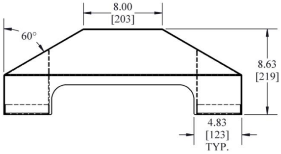
SCE-24PEBASE SCE-24PEBASESS
