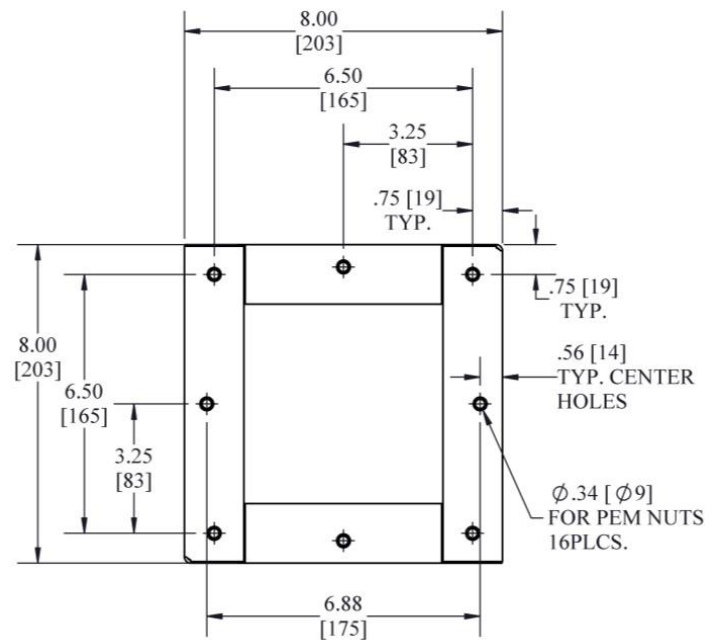
HOLES AND PEMS TYP. TOP AND BOTTOM
