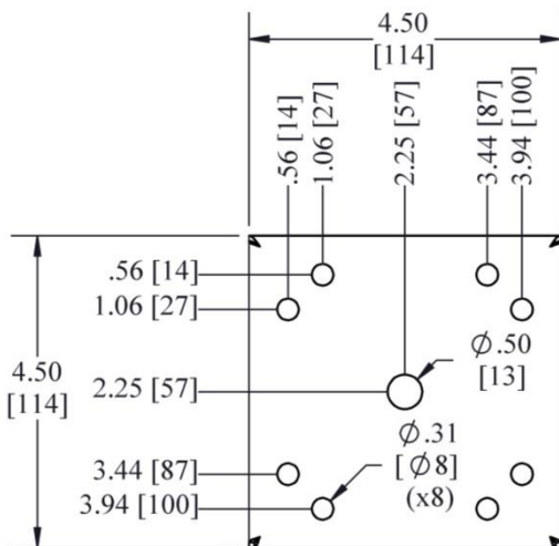
BASE PAD (4 PCS. PER UNIT)
