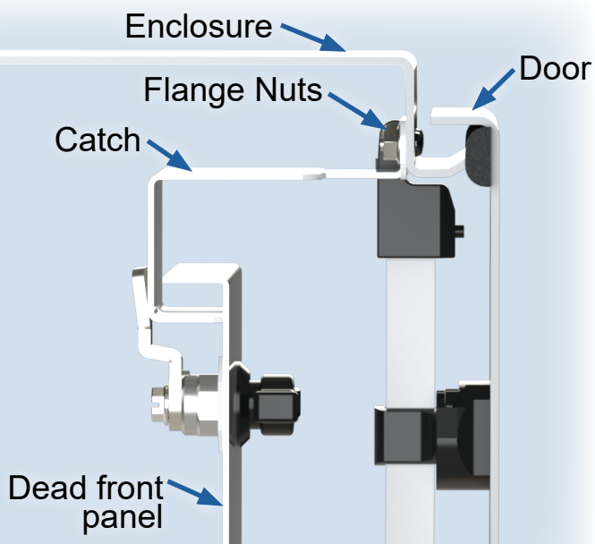
Section Z-Z
