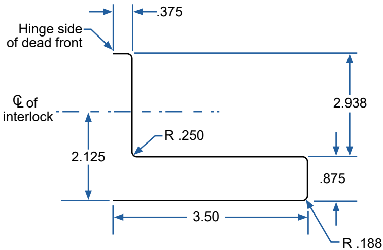
"K" Detail (Not to scale) Mechanical interlock arm clearance cutout required on the hinge side of dead front. Cutout required only when new plastic interlock is used.
