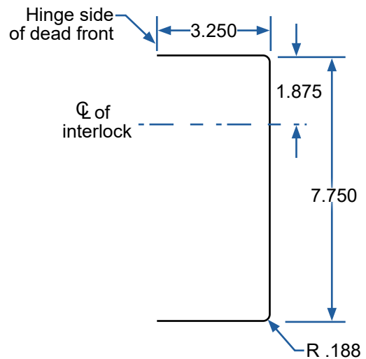
"K" Detail (Not to scale) Mechanical interlock arm clearance cutout required on the hinge side of dead front. Cutout required only when old metal interlock is used.
